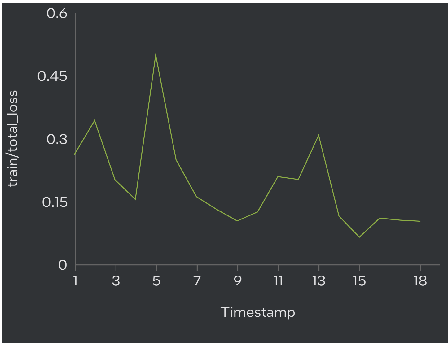
train/total_loss
