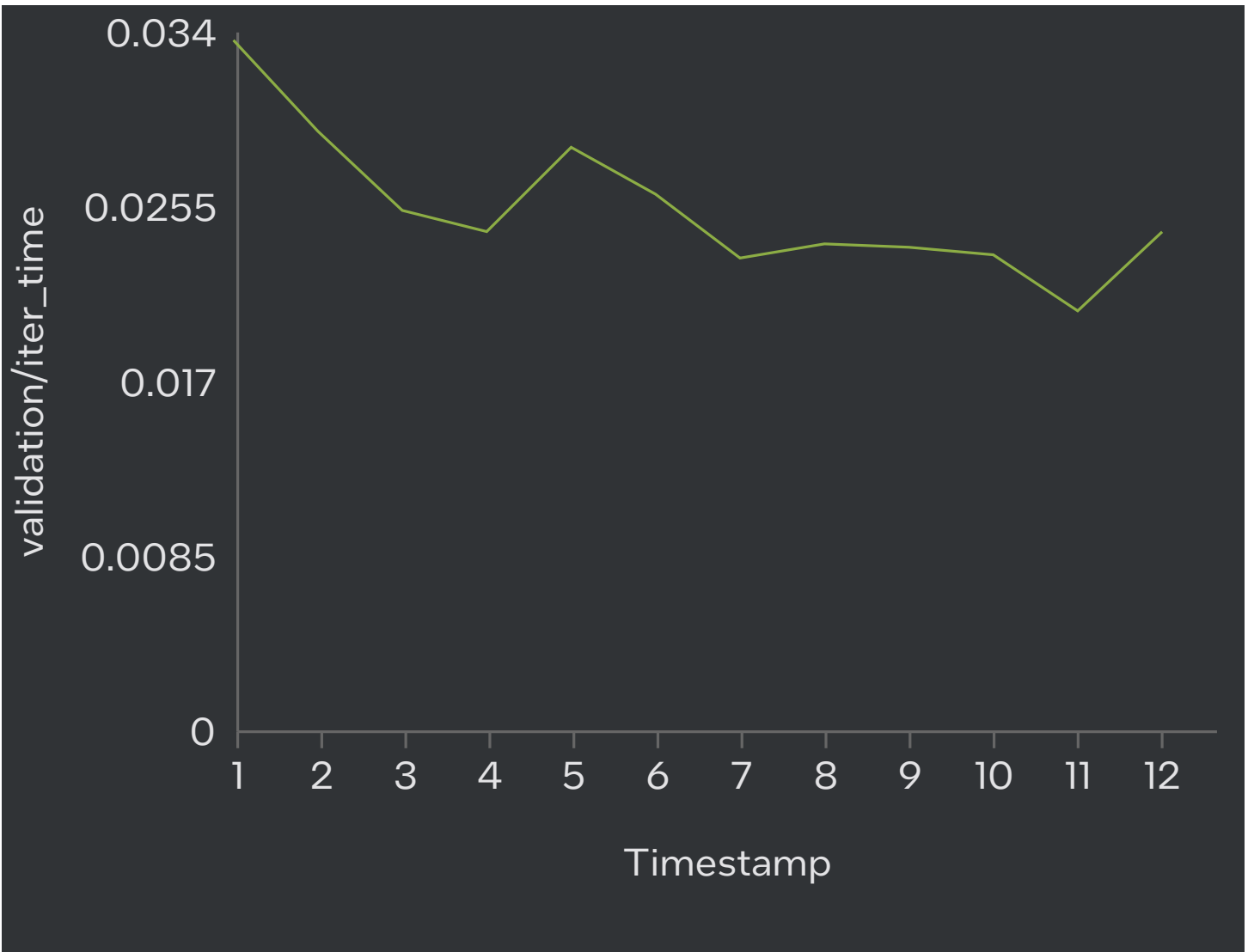
validation/iter_time
