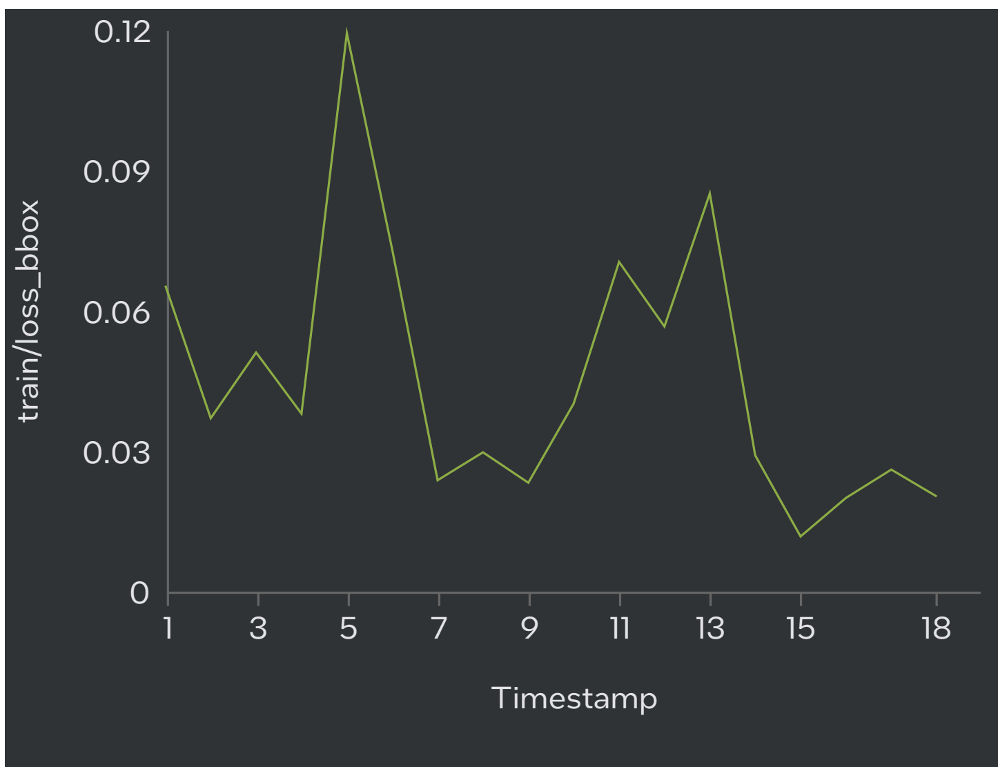
train/loss_bbox
