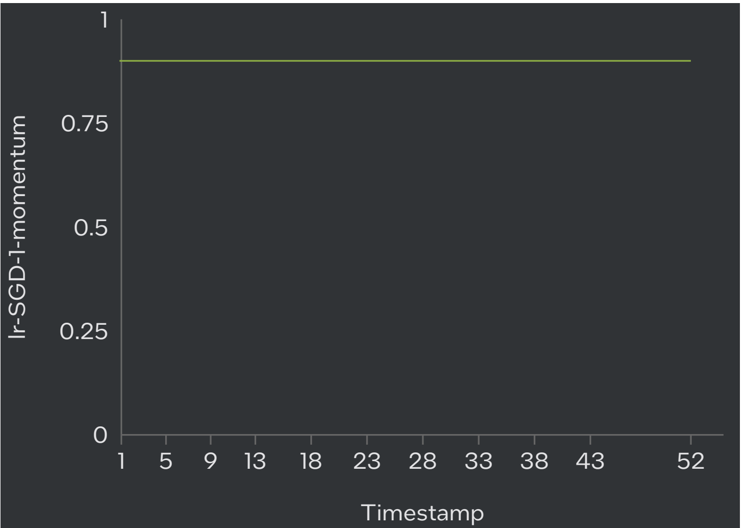
lr-SGD-l-momentum
