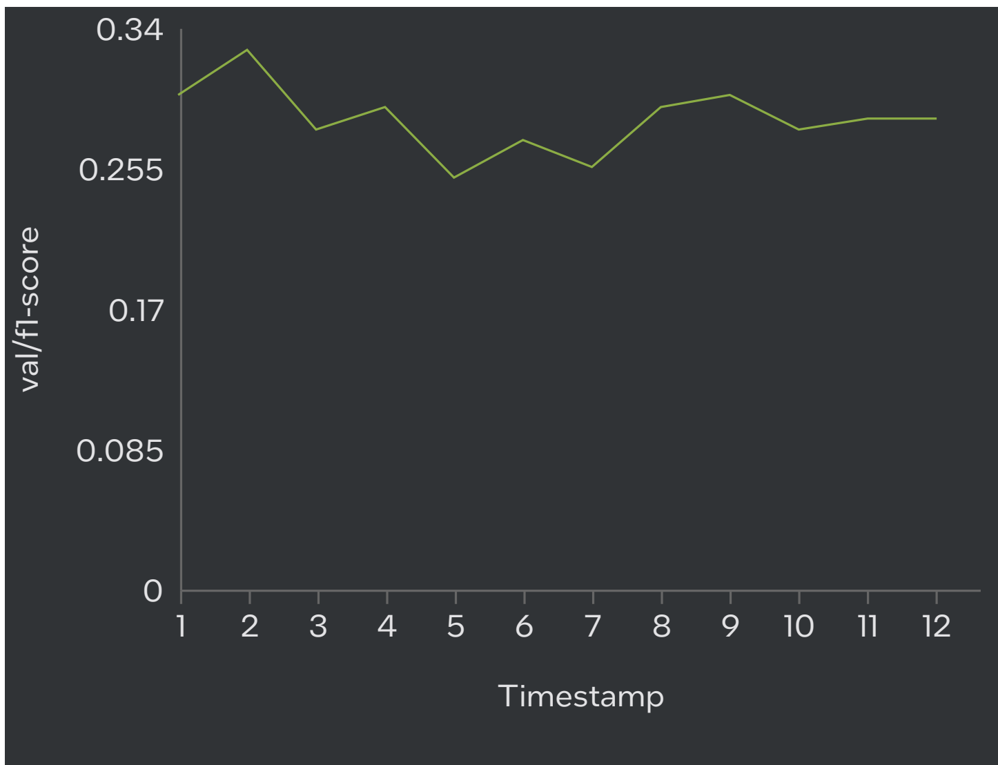
val/f1-score
