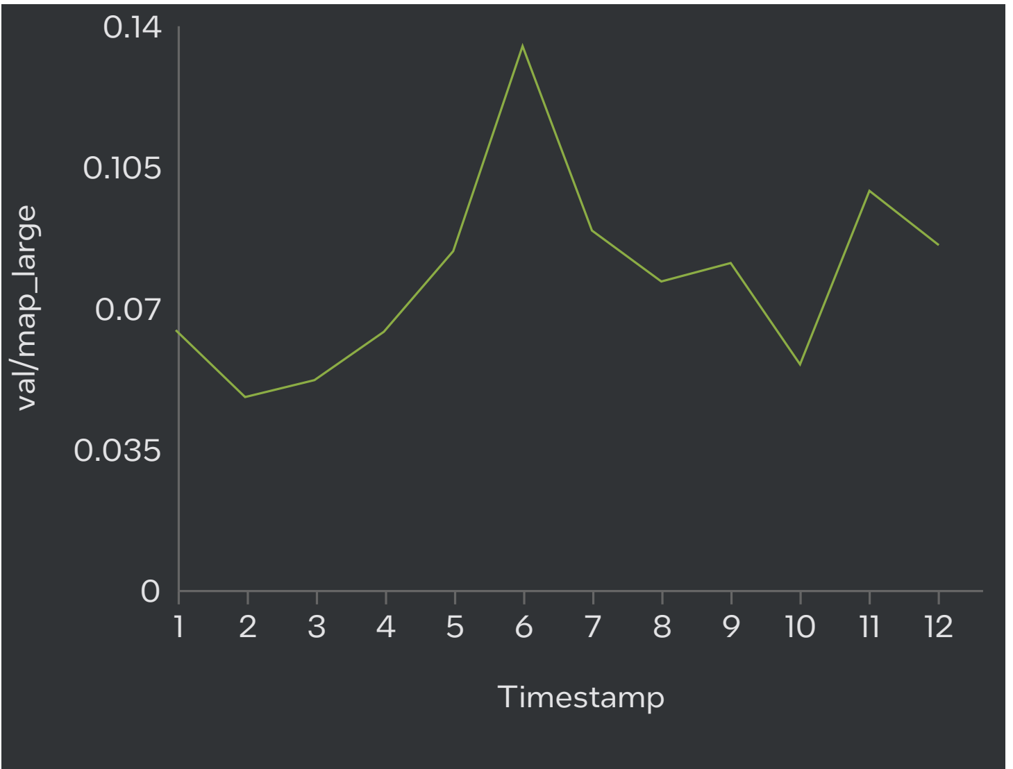
val/map_large
