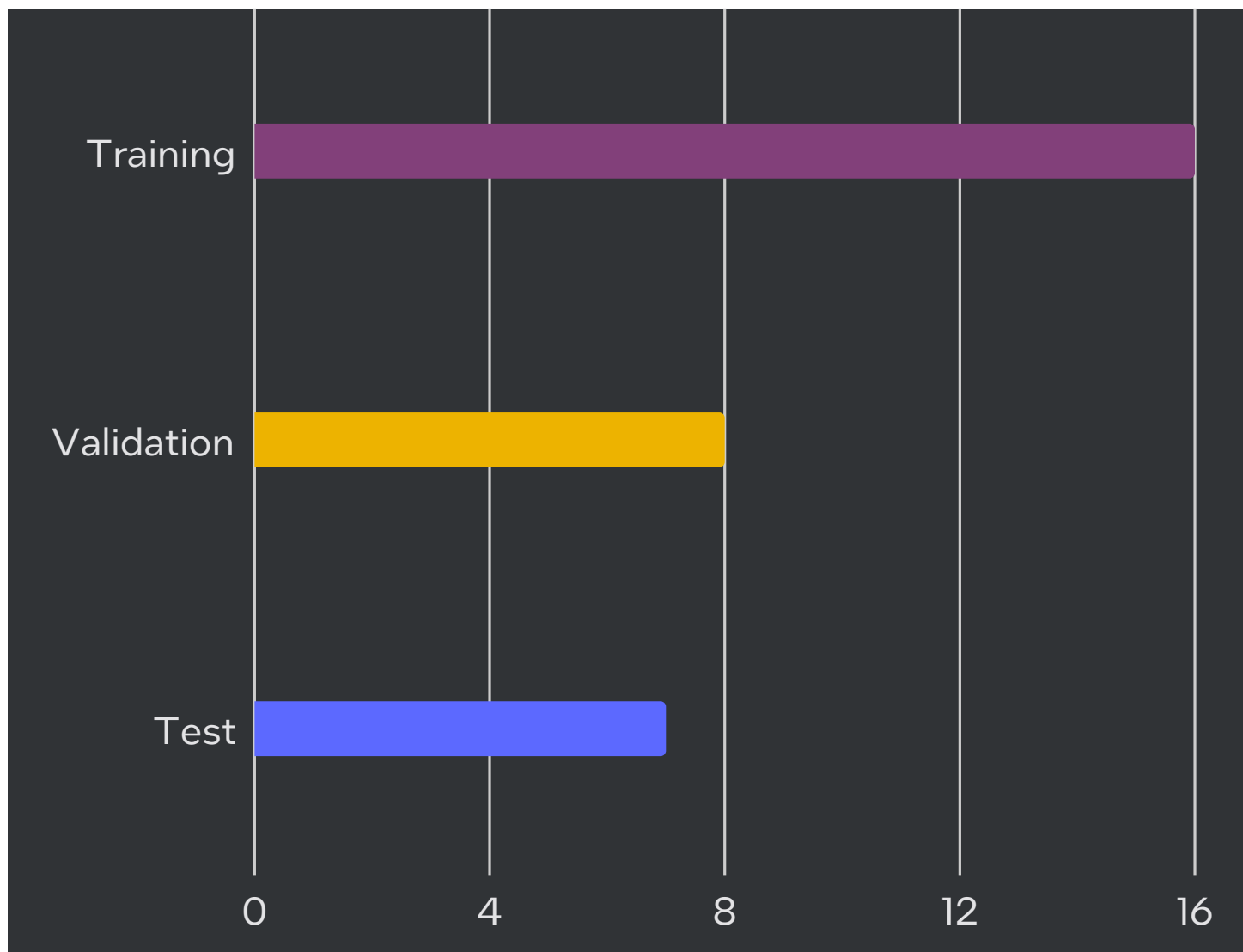
Dataset split
