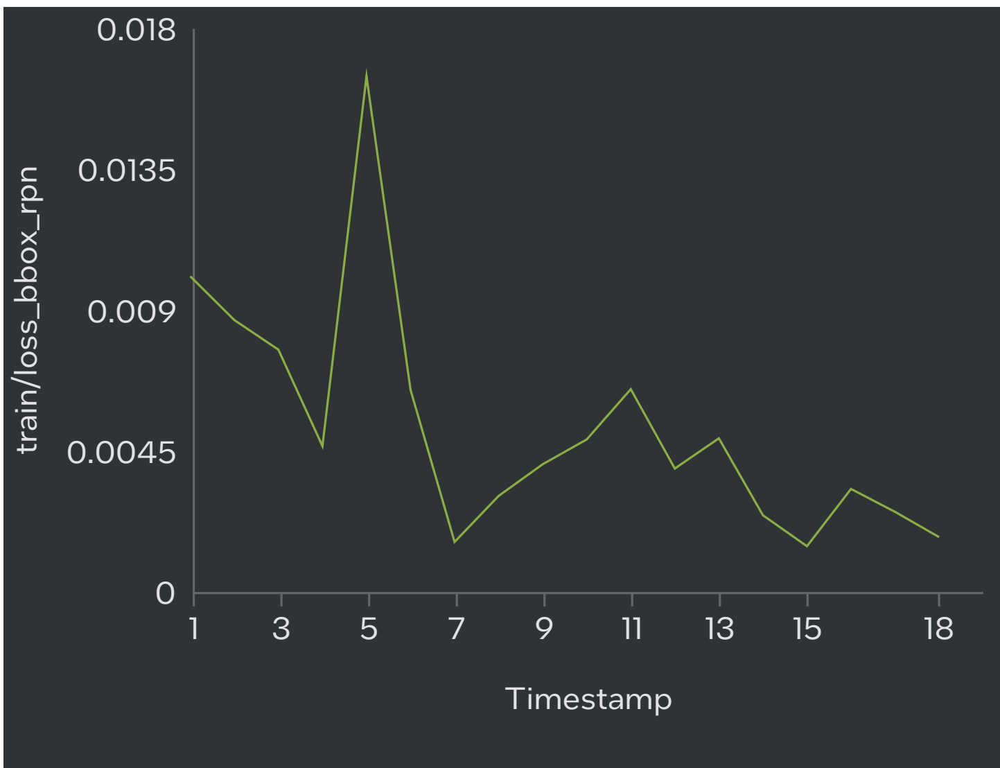
train/loss_bbox_rpn
