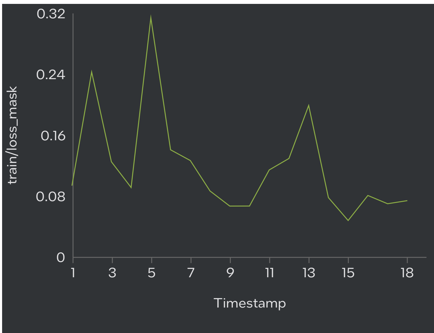
train/loss_mask
