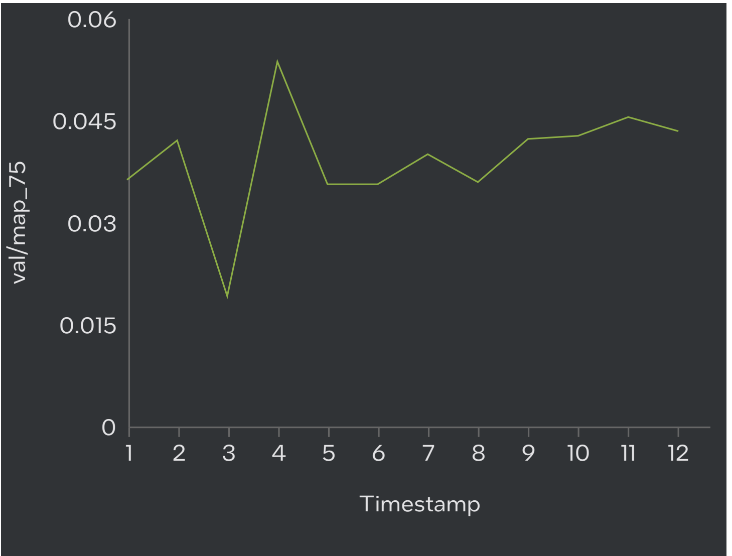
val/map_75
