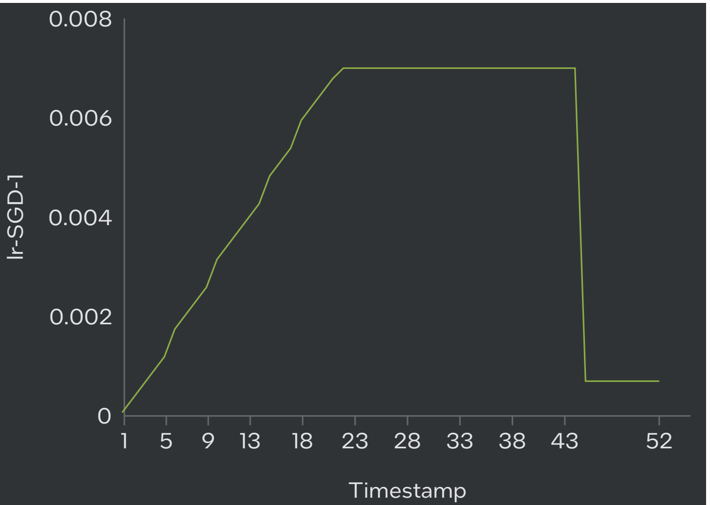
lr-SGD-1
