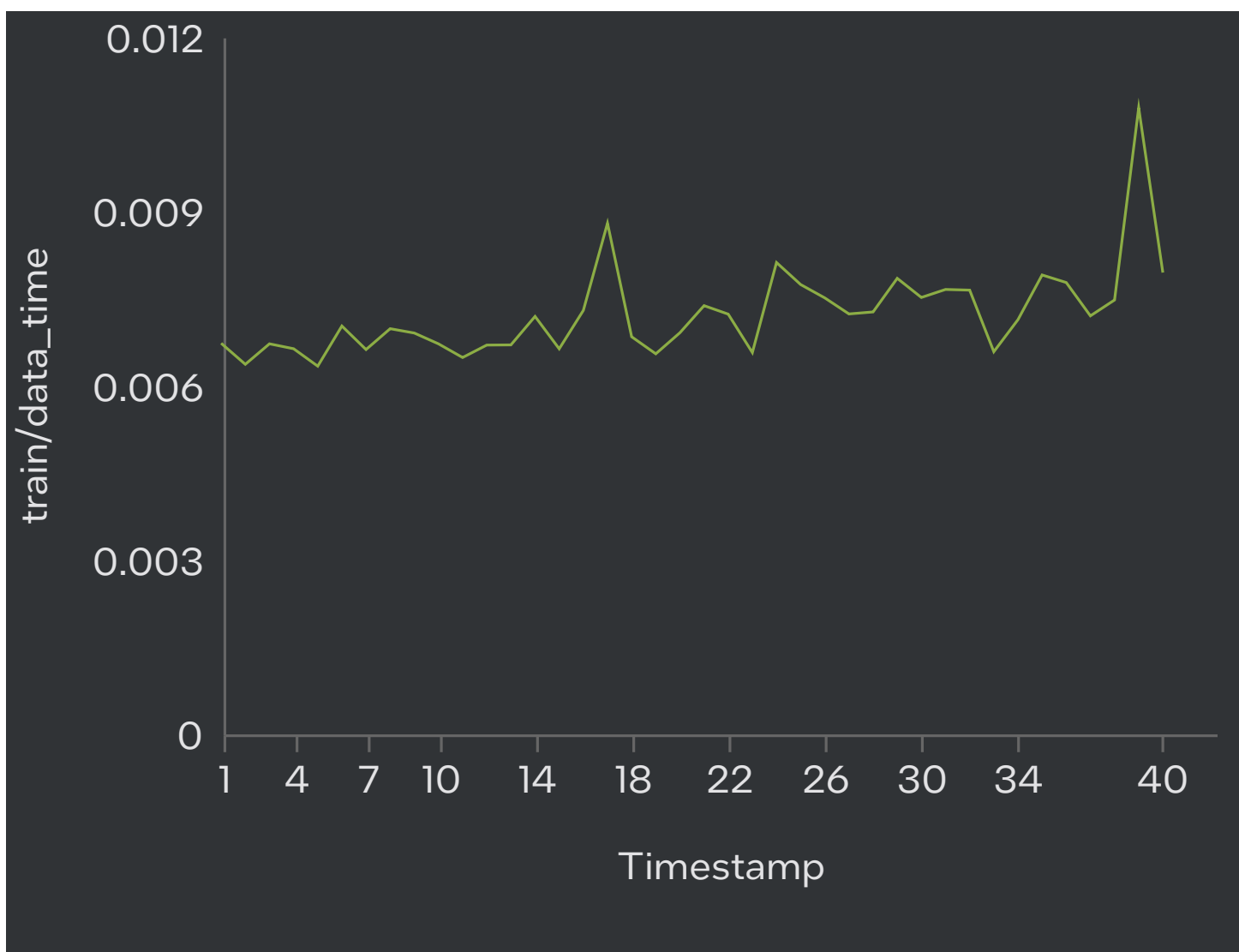
train/data_time
