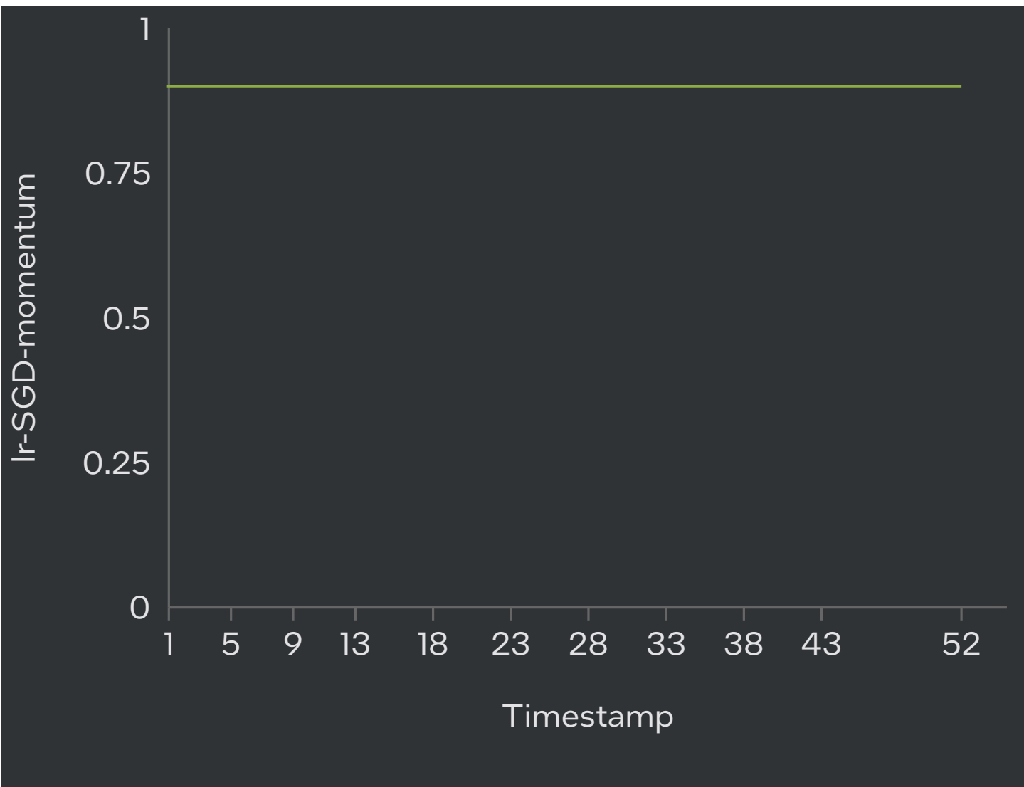
lr-SGD-momentum
