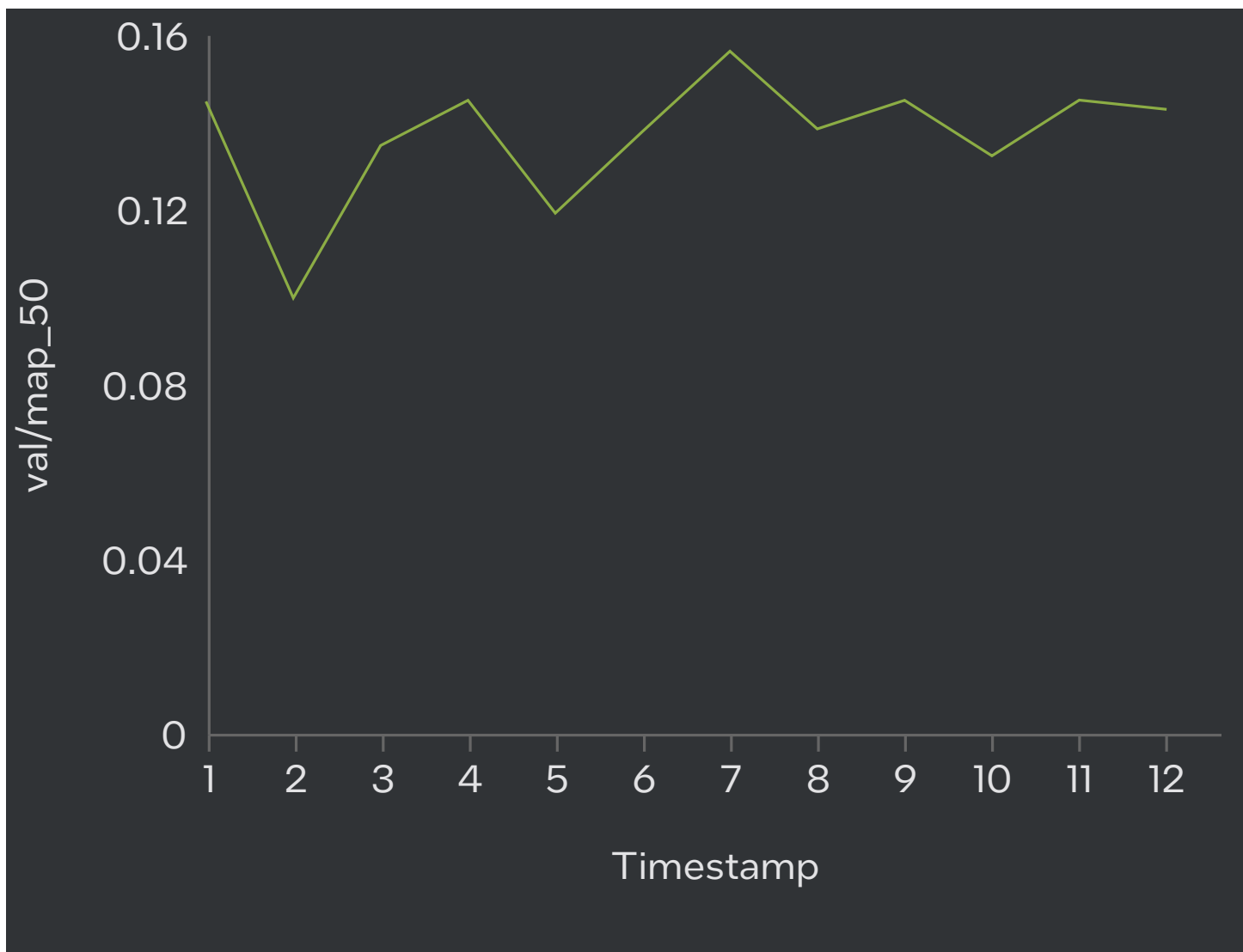
val/map_50
